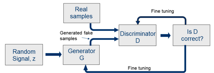
Fig. 7. Structure of generative adversarial network.
